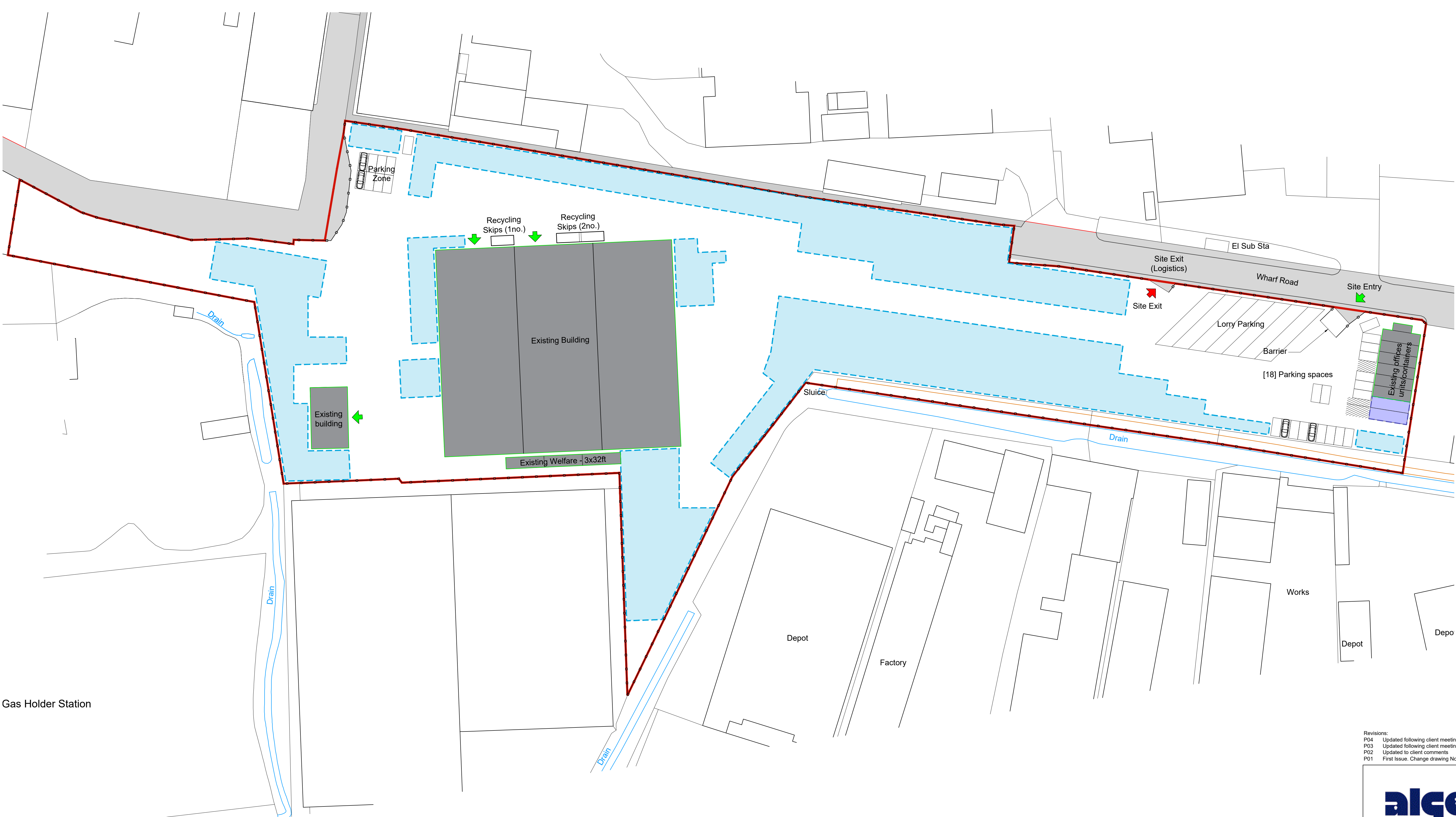
Site Layout Plan as Existing 1:500
