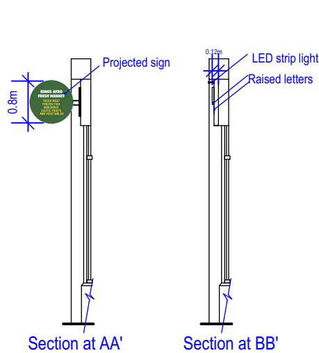
Section through Entrance
