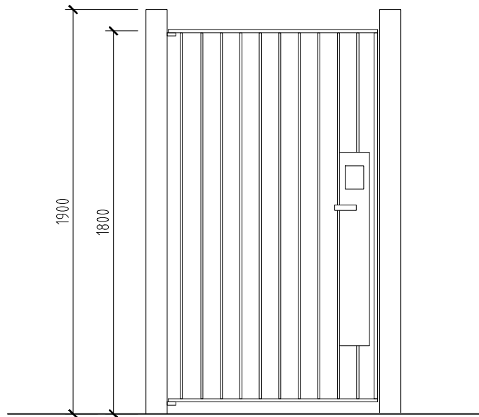
Proposed metal railing and cycle store access gate Scale 1:25
