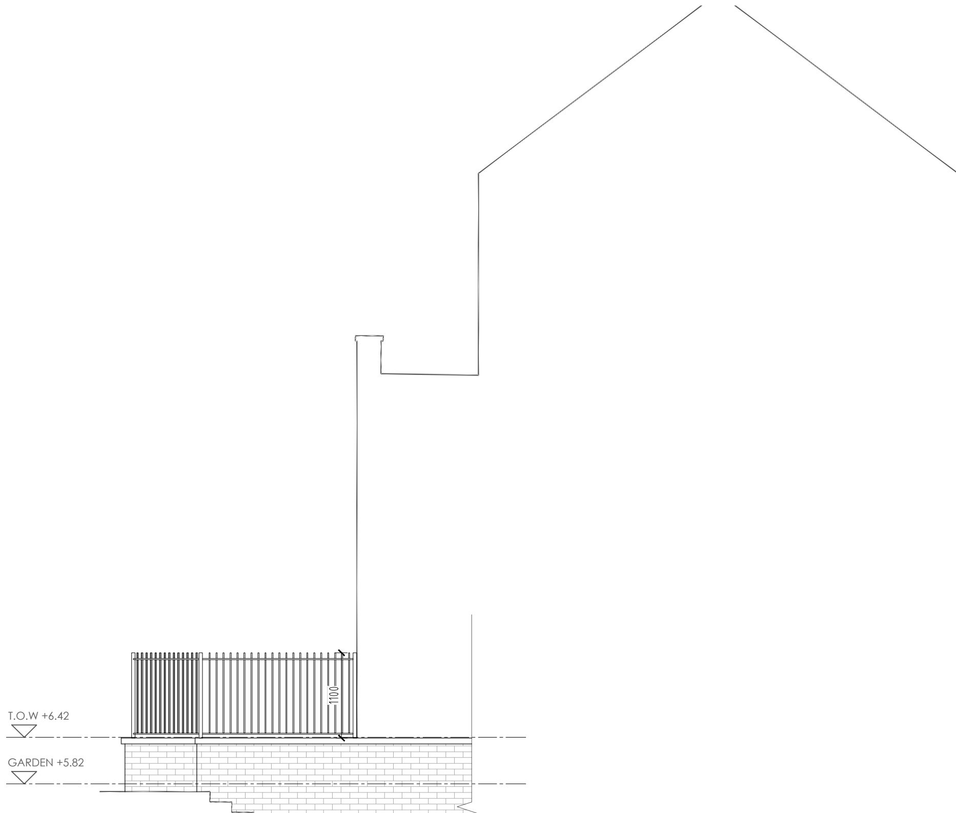
Proposed brick retaining wall with metal railing in front of new build Scale 1:50
