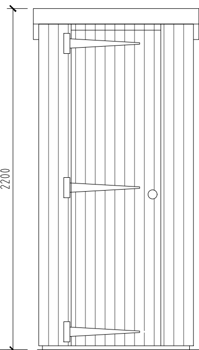
Front
