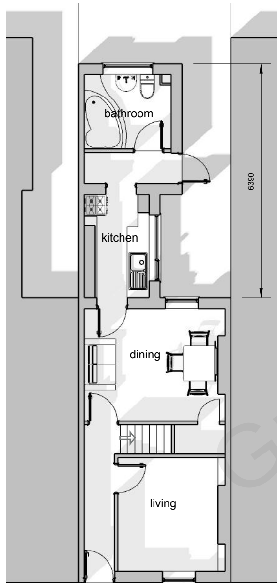
b ground floor plan 002 scale: 1:100 0 1 2m
