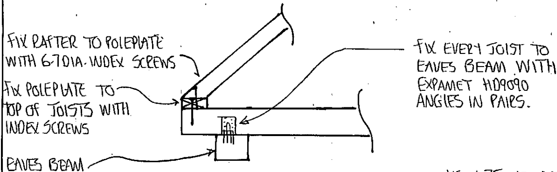
DETAIL 1
