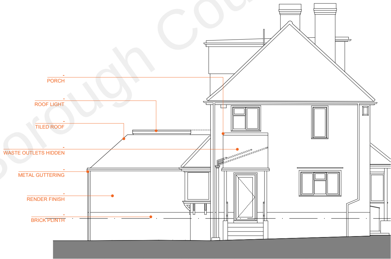
02 PROPOSED NORTH WEST ELEVATION 1:100 @ A3
