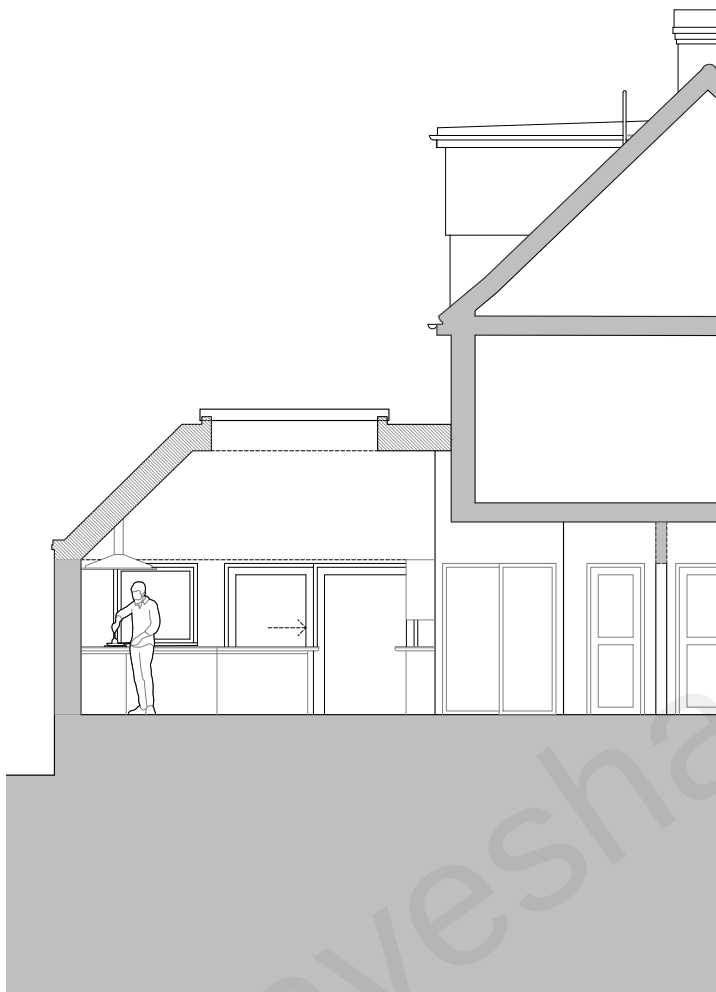
01 PROPOSED SECTION AA 1:100 @ A3
