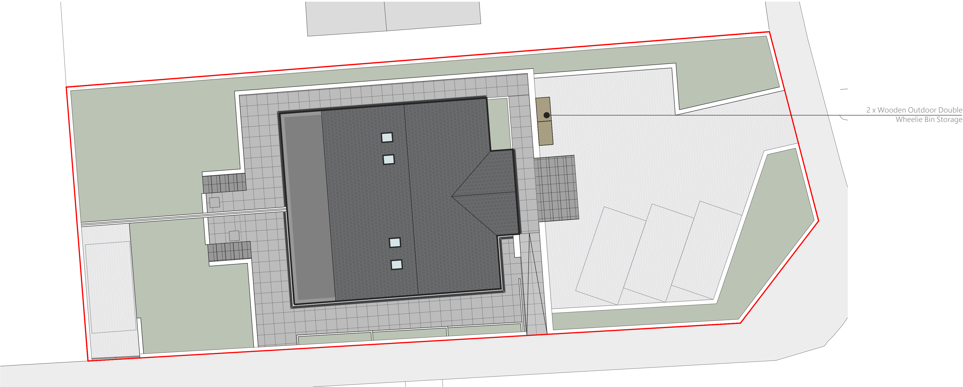
Proposed Block Plan 1:100
