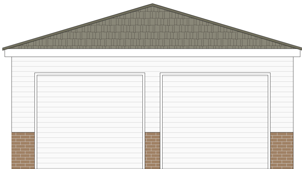
West Elevation
