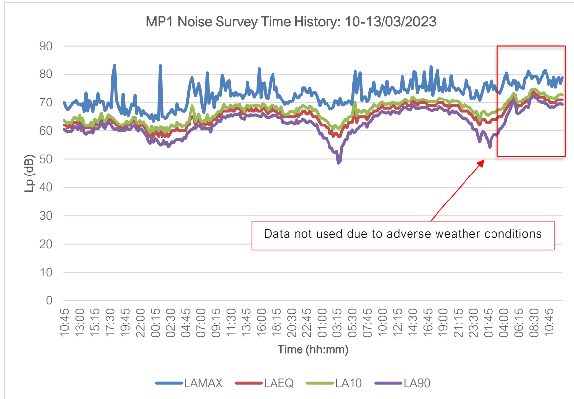
Figure 10 – MP1 Noise Survey Time History
