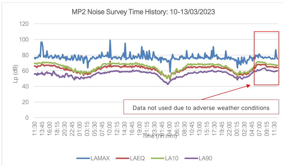
Figure 11 – MP2 Noise Survey Time History
