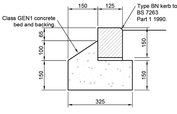
BN KERB DETAIL (Scale 1:10)
