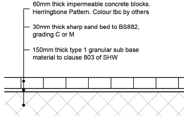
TYPE C - BLOCK PAVING FOOTPATH CONSTRUCTION (Scale 1:20)
