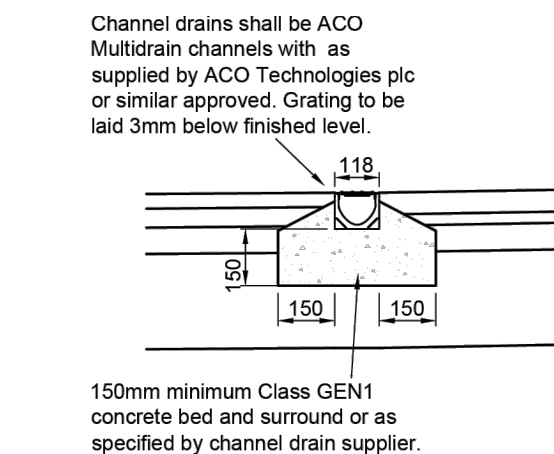
ACO CHANNEL CAR PARK / DRIVEWAY DRAIN DETAIL (Scale 1:20)
