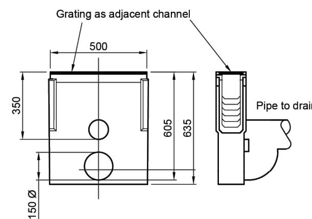
ACO UNIVERSAL SUMP DETAIL (Scale 1:20)
