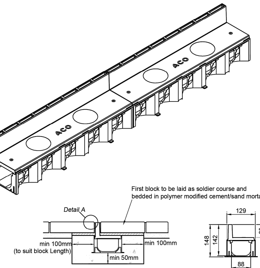
HEXDRAIN BRICKSLOT THRESHOLD CHANNEL (Scale 1:10)
