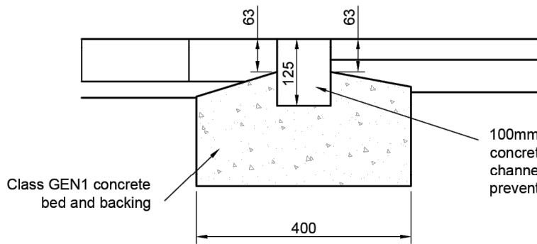
CONCRETE CHANNEL DETAIL FOR DEMARCATION - NON DISHED (Scale 1:10)
