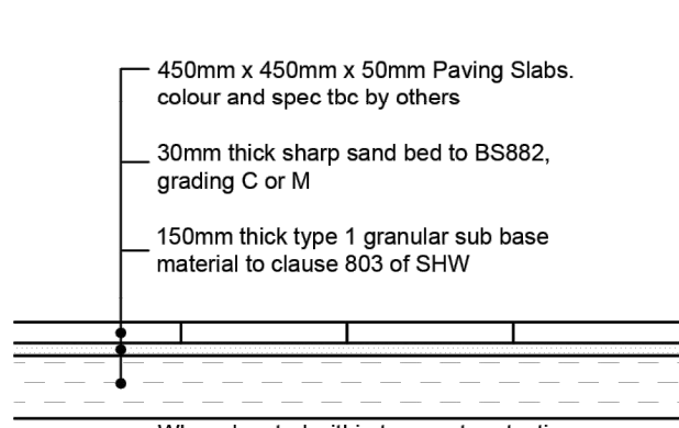
TYPE B - PAVING SLAB PATIO / FOOTPATH CONSTRUCTION (Scale 1:20)
