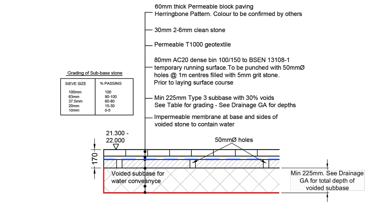
TYPE A - PERMEABLE BLOCK PAVING CAR PARK CONSTRUCTION WITH TEMPORARY RUNNING COURSE (Scale 1:20)
