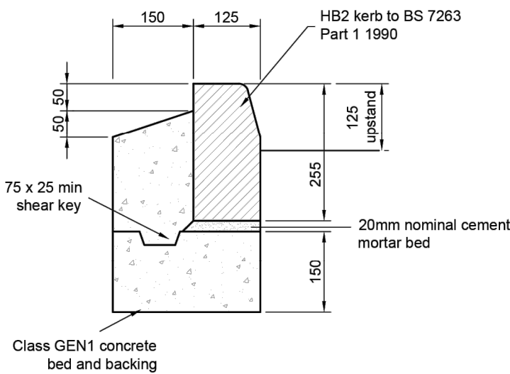
HB2 KERB DETAIL (Scale 1:10)
