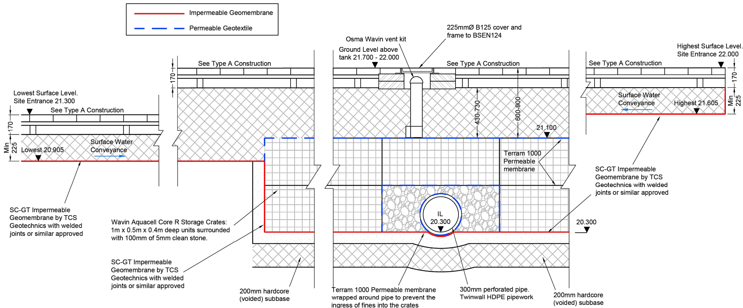
CRATE STORAGE DETAIL (Scale 1:20)
