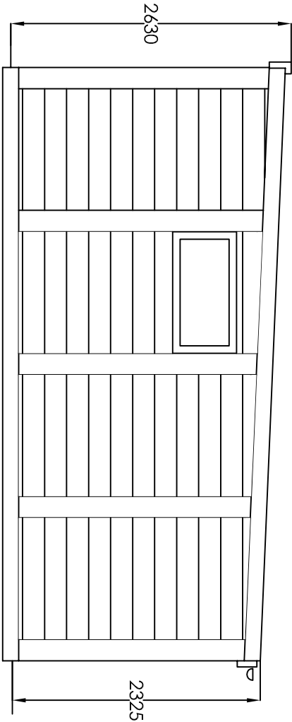
SIDE ELEVATION
