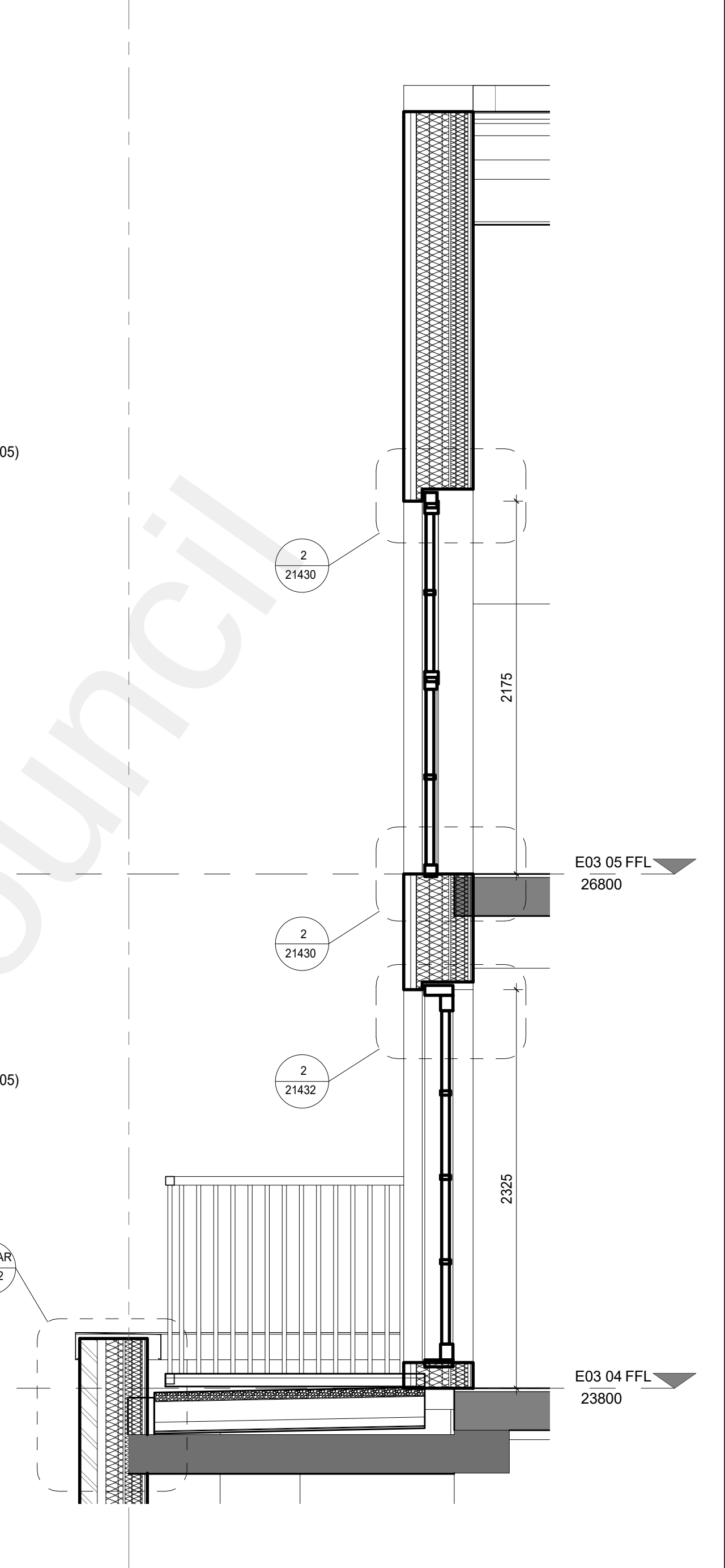
4 E03 BAY SECTION NORTH LEVEL 04-05 1:25
