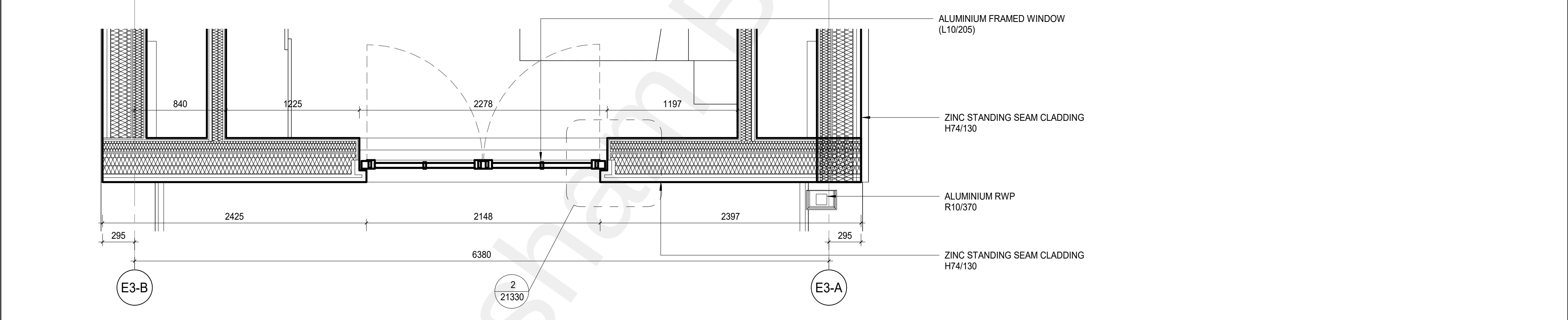
4 E03 BAY SECTION NORTH LEVEL 04-05 1:25
