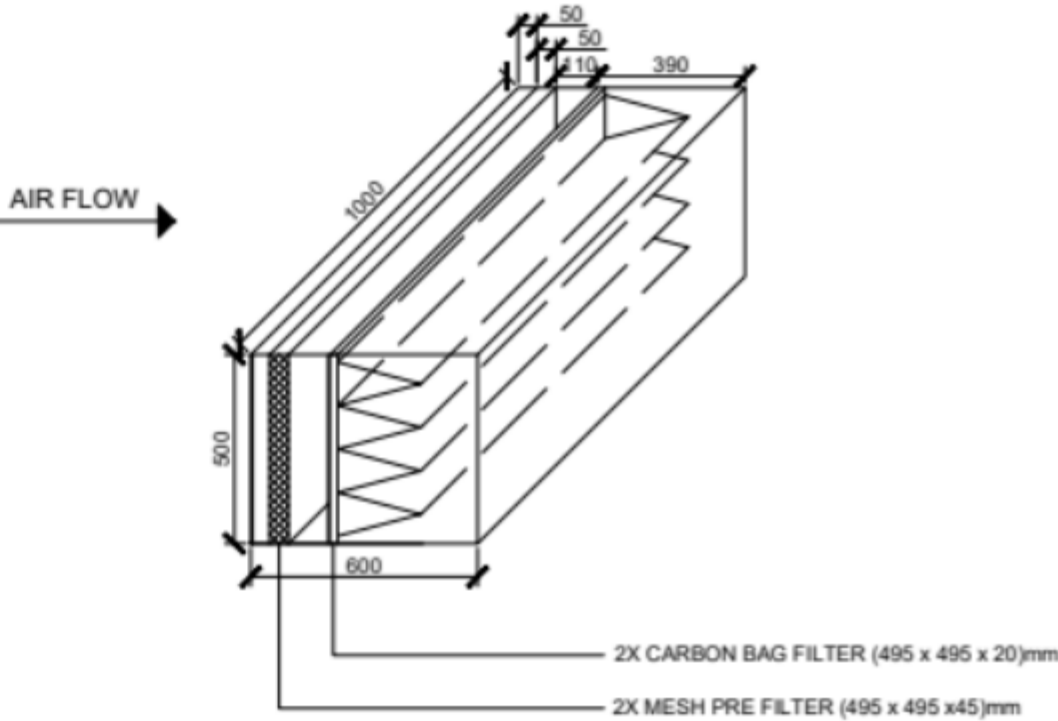
ODOR CONTROL SYSTEM FILTRATION UNIT
