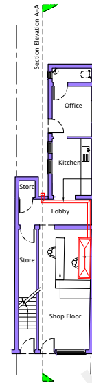
Proposed Takeaway Plan
