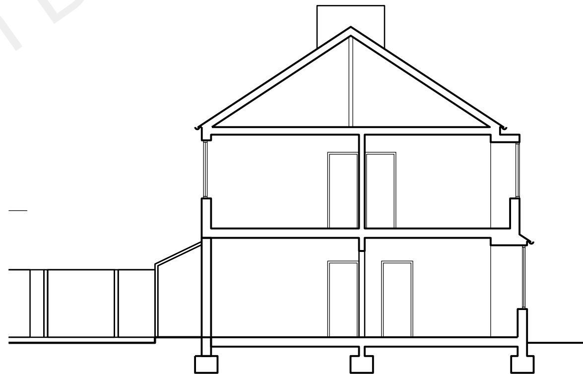
04 Section through 45 Woodfield Av. (looking North) 1:100
