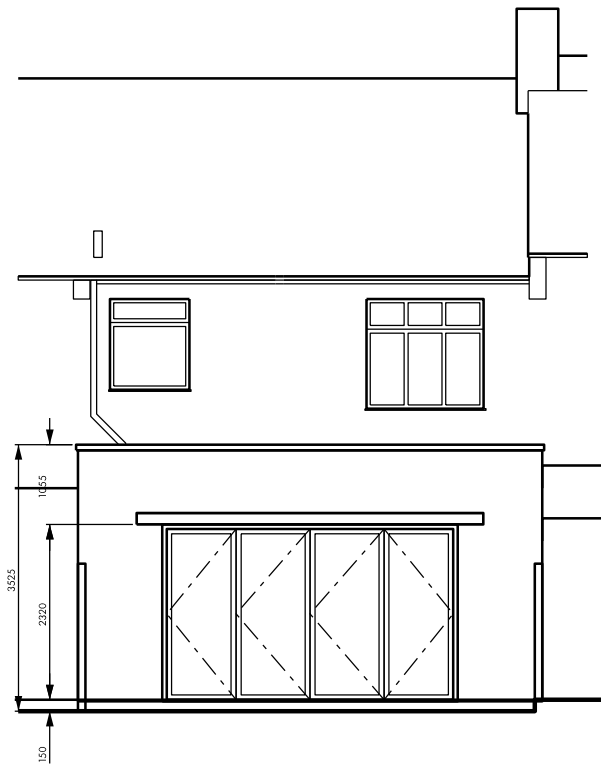
01 Rear (West) Elevation 1:100
