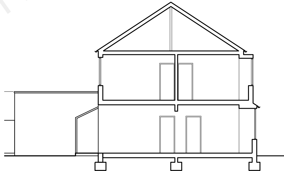
04 Section through 45 Woodfield Av. (looking North) 1:100
