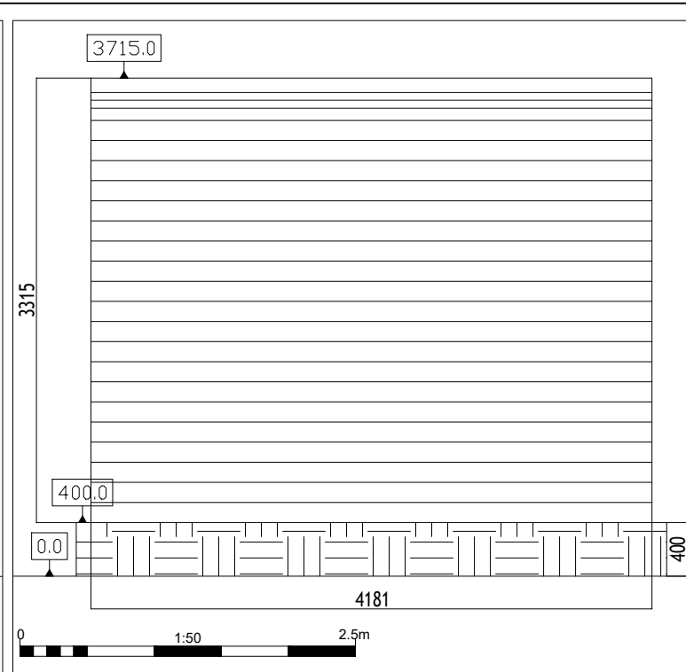
Left Elevation (C:C)
