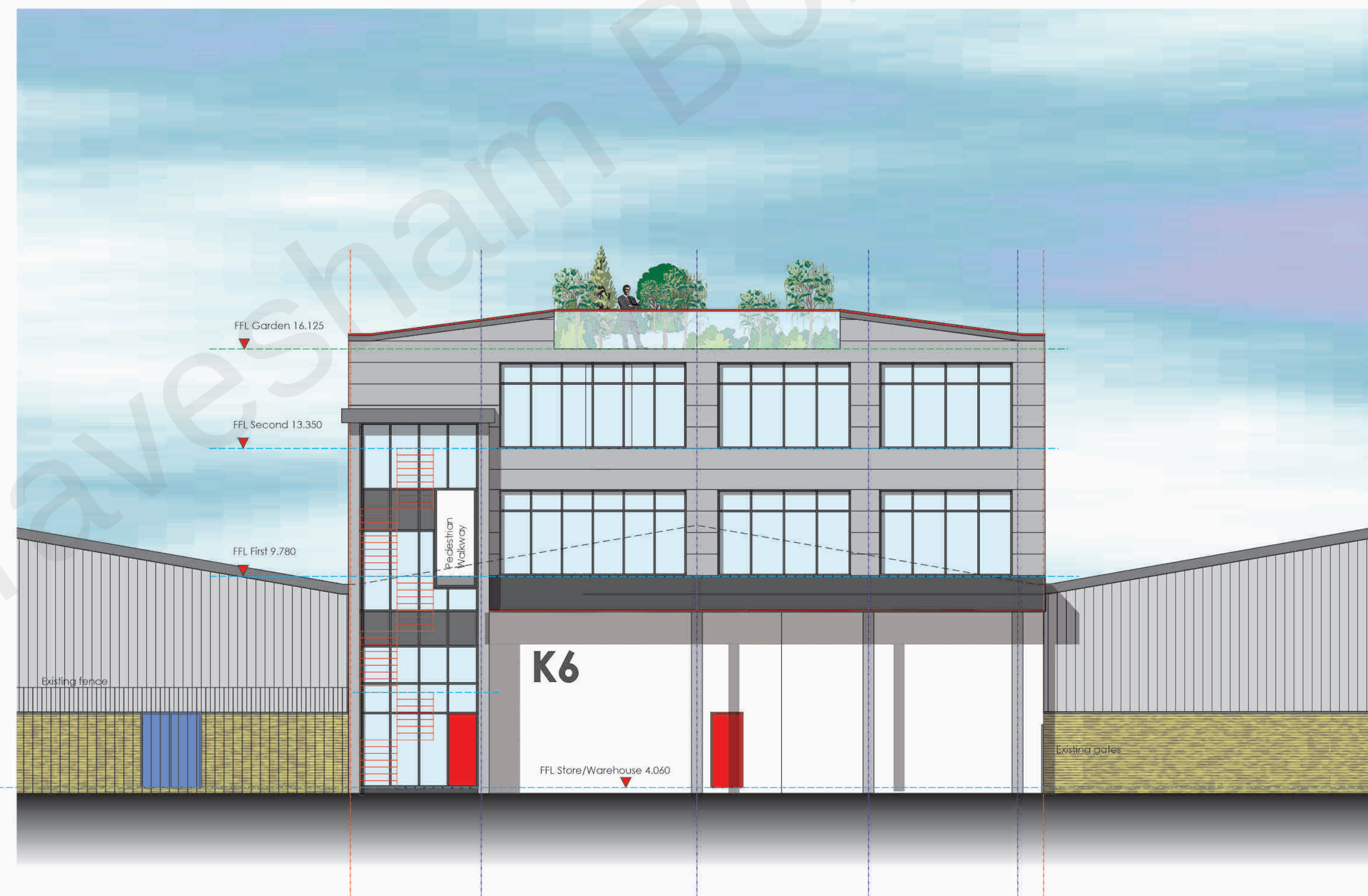
Rear Elevation - 1:100 SOUTH WEST
