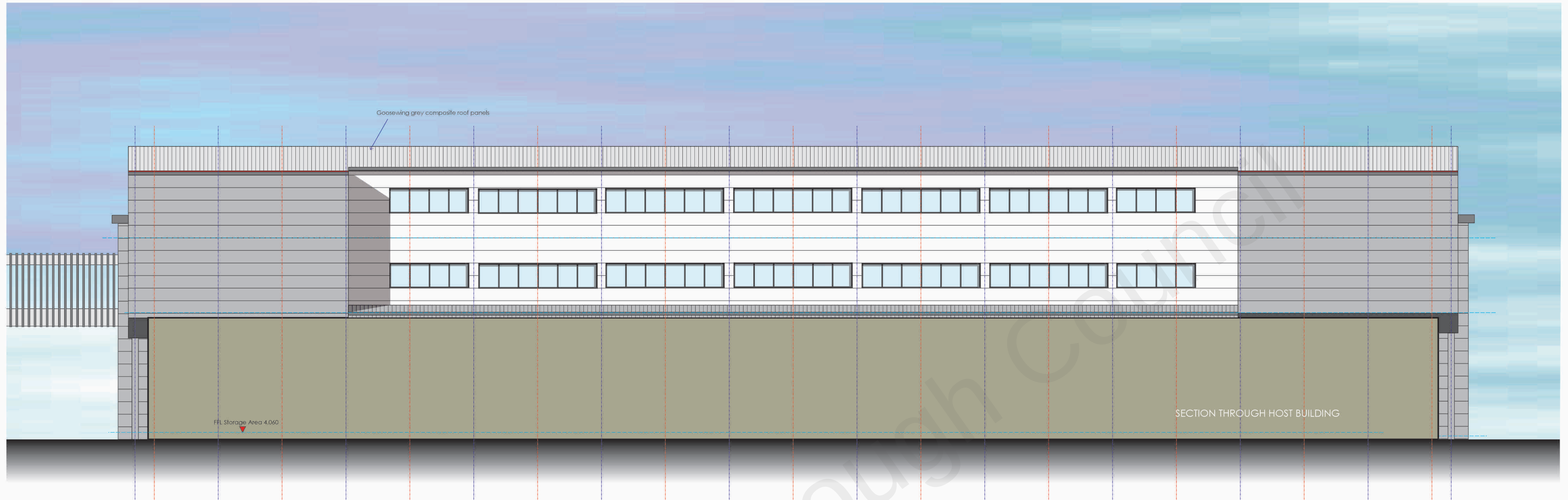
Proposed Side Elevation - 1:100 NORTH WEST
