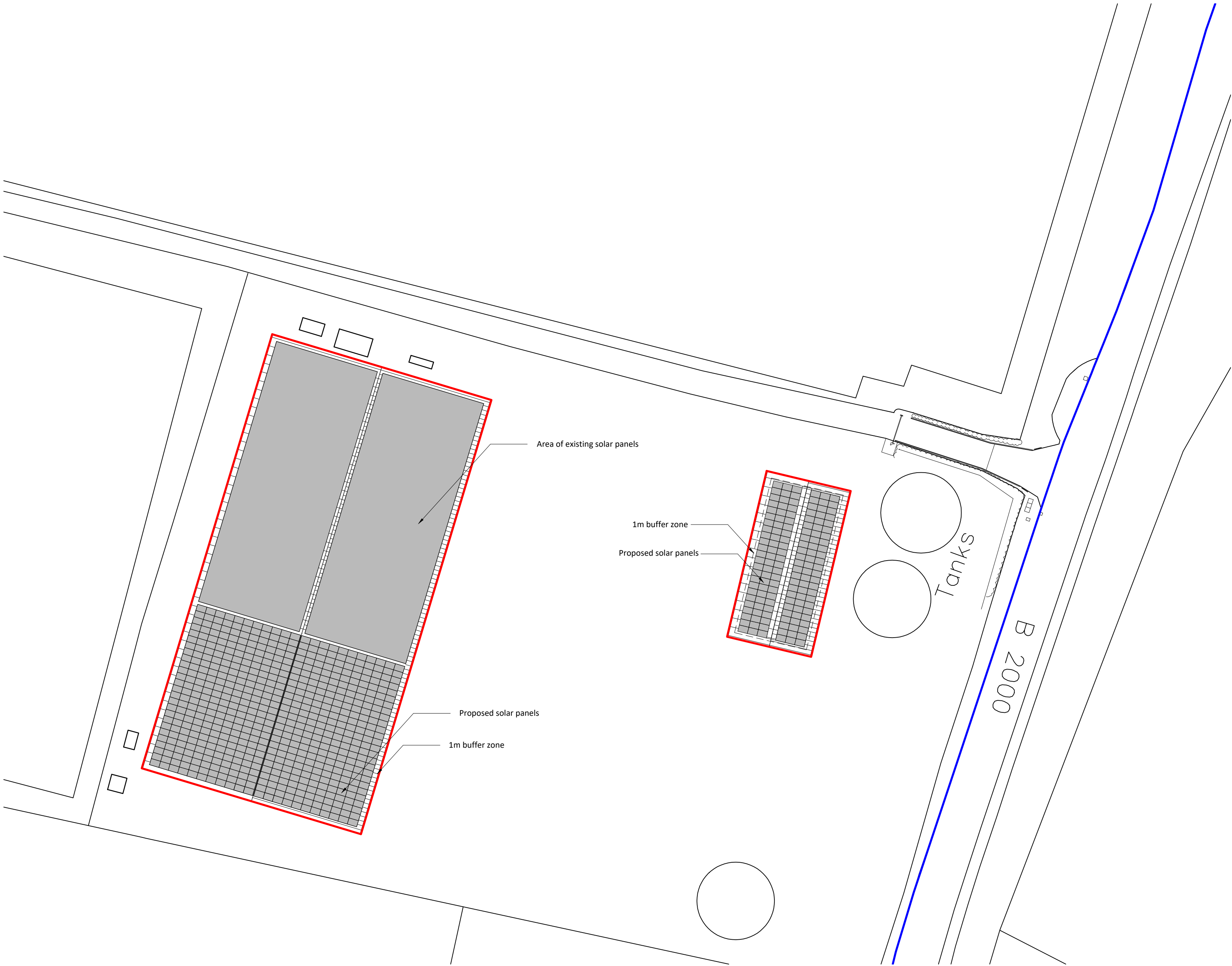
Proposed Block Plan 1:500
