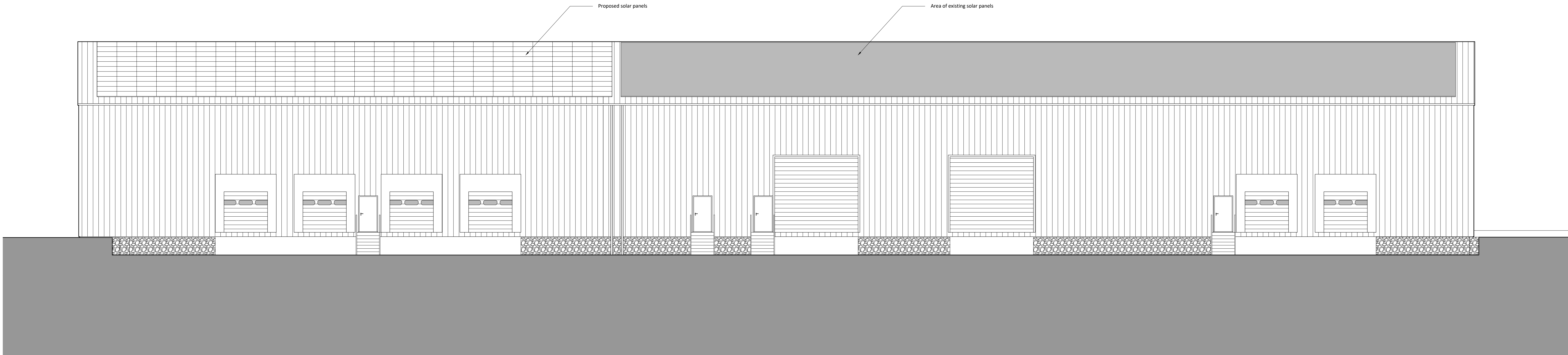
Proposed Front (South-East) Elevation 1:100
