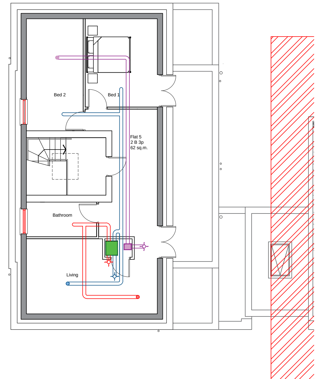
Second Floor
