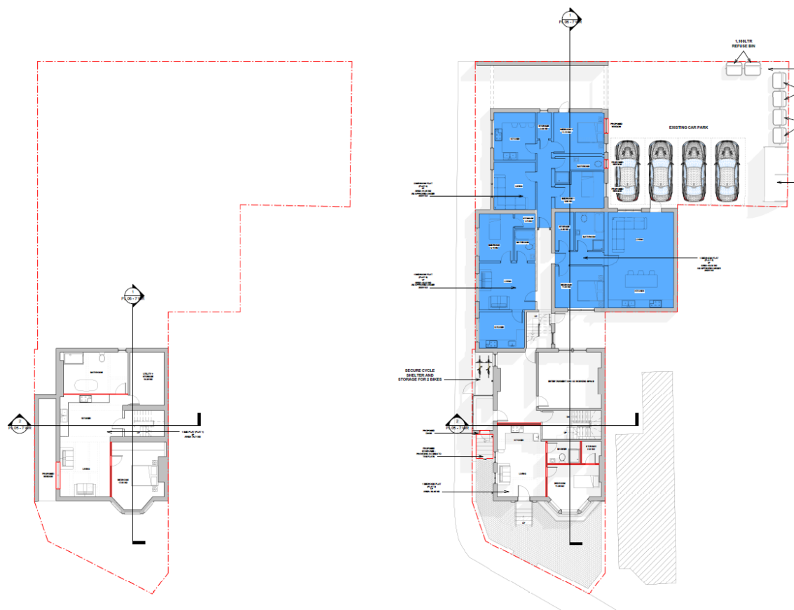
Figure 4: Proposed basement and ground floor plan
