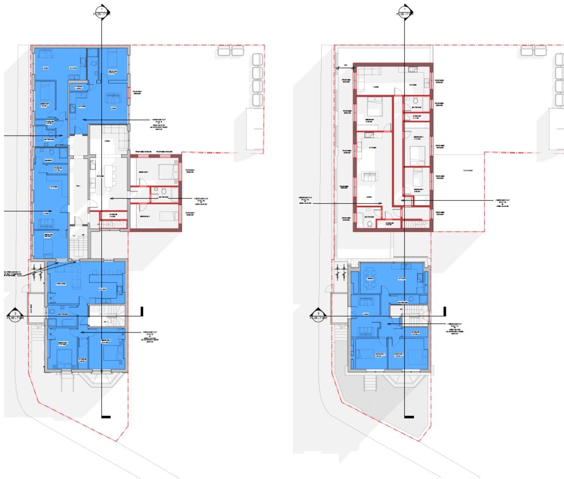
Figure 5: First and top floor plan
