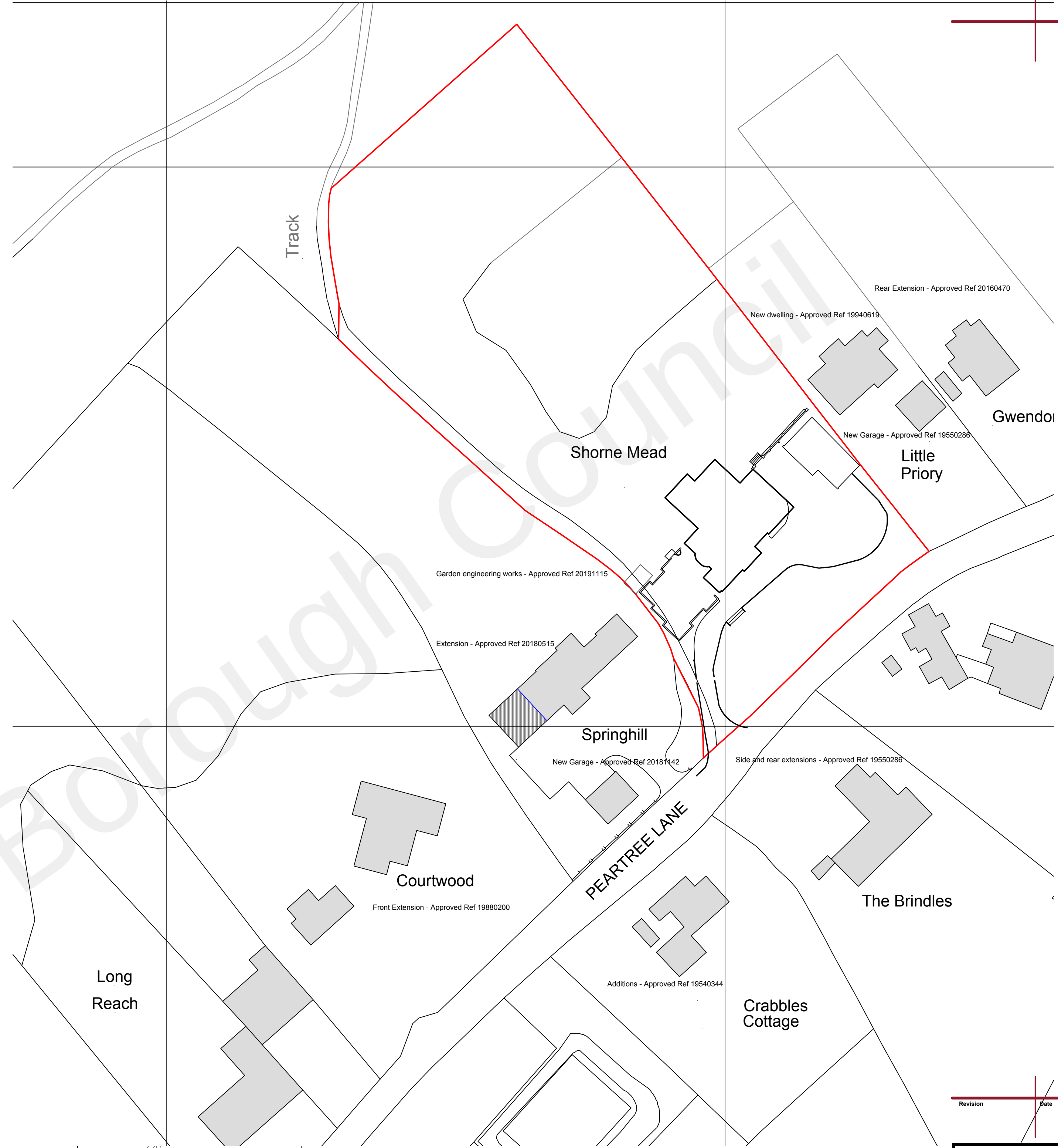
PROPOSED BLOCK PLAN 1-500
