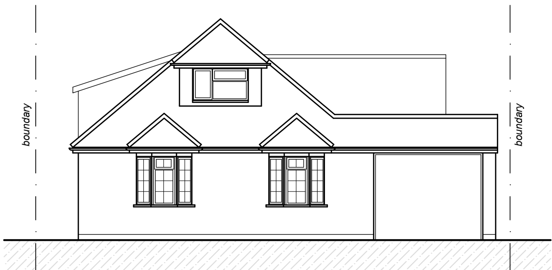
FRONT ELEVATION (1:100)
