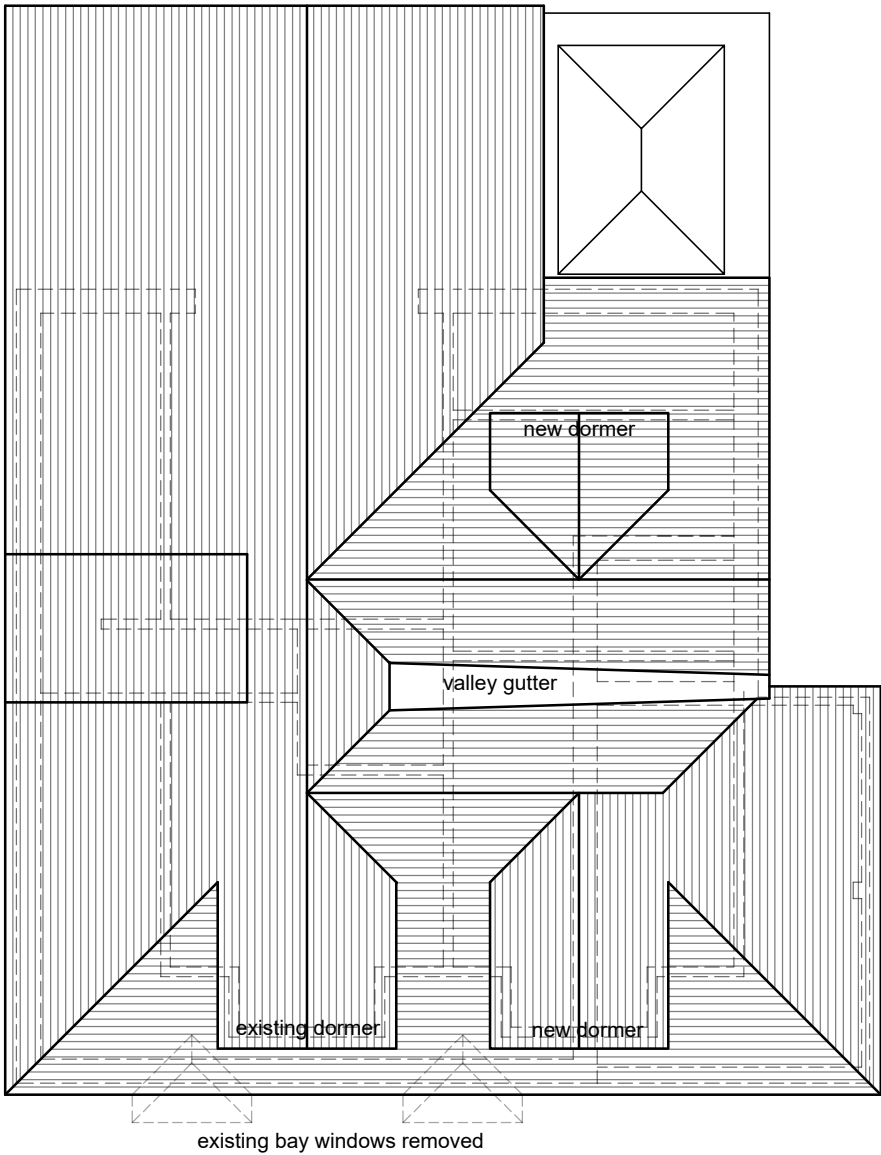
ROOF PLAN (1:100)
