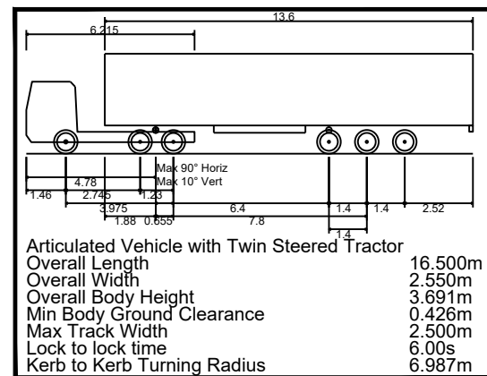
Vehicle Profile
