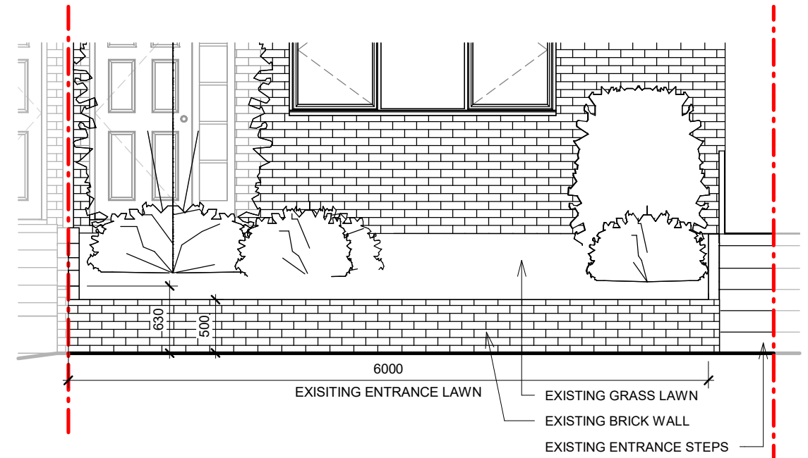
2 FRONT ELEVATION 1 : 50 2.5 m 1m 2.5m 1:50
