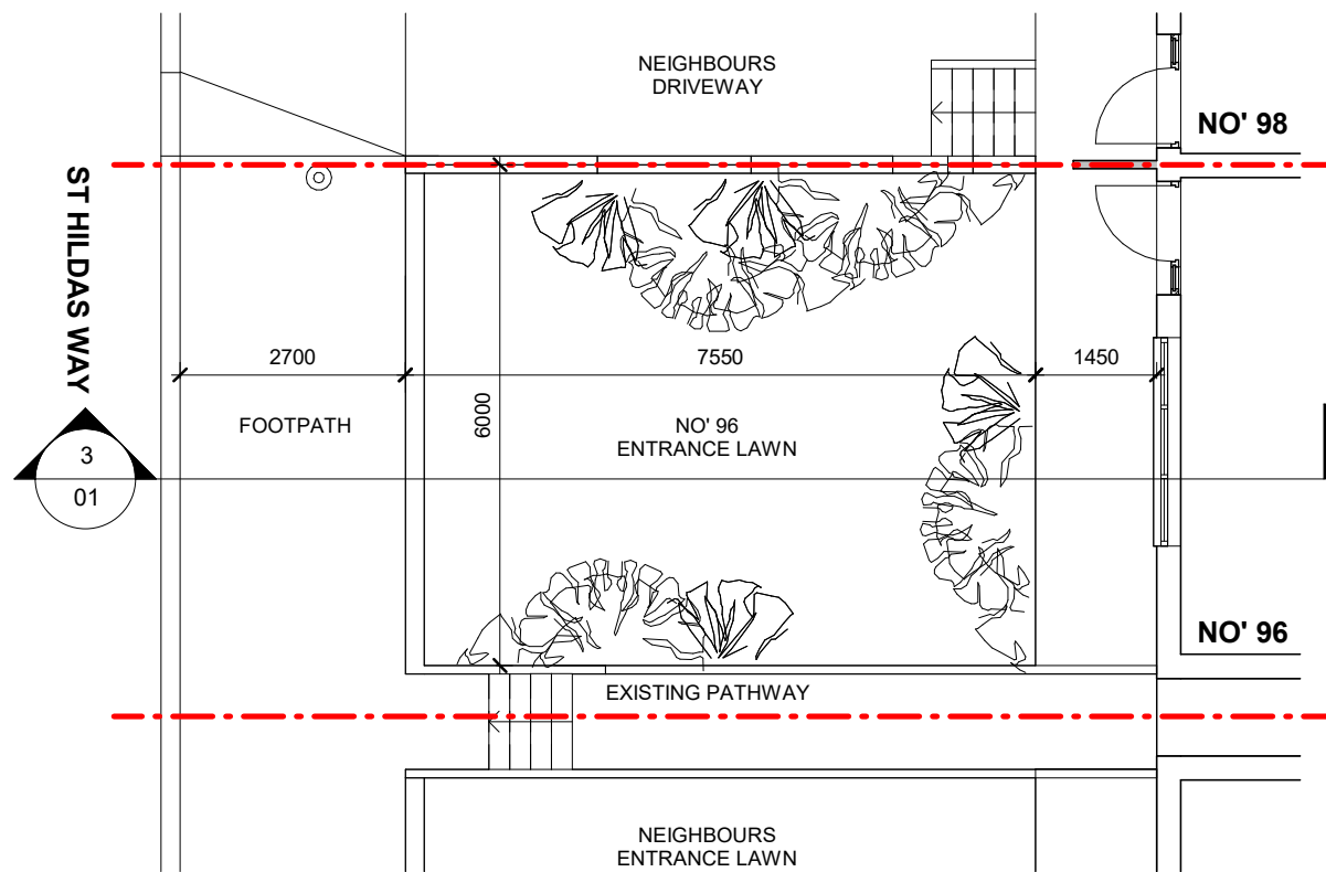
1 PRE EXISTING GROUND FLOOR PLAN 1 : 100
