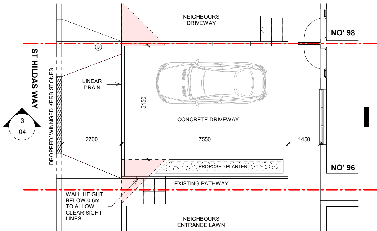
1 PROPOSED GROUND FLOOR PLAN 1:100
