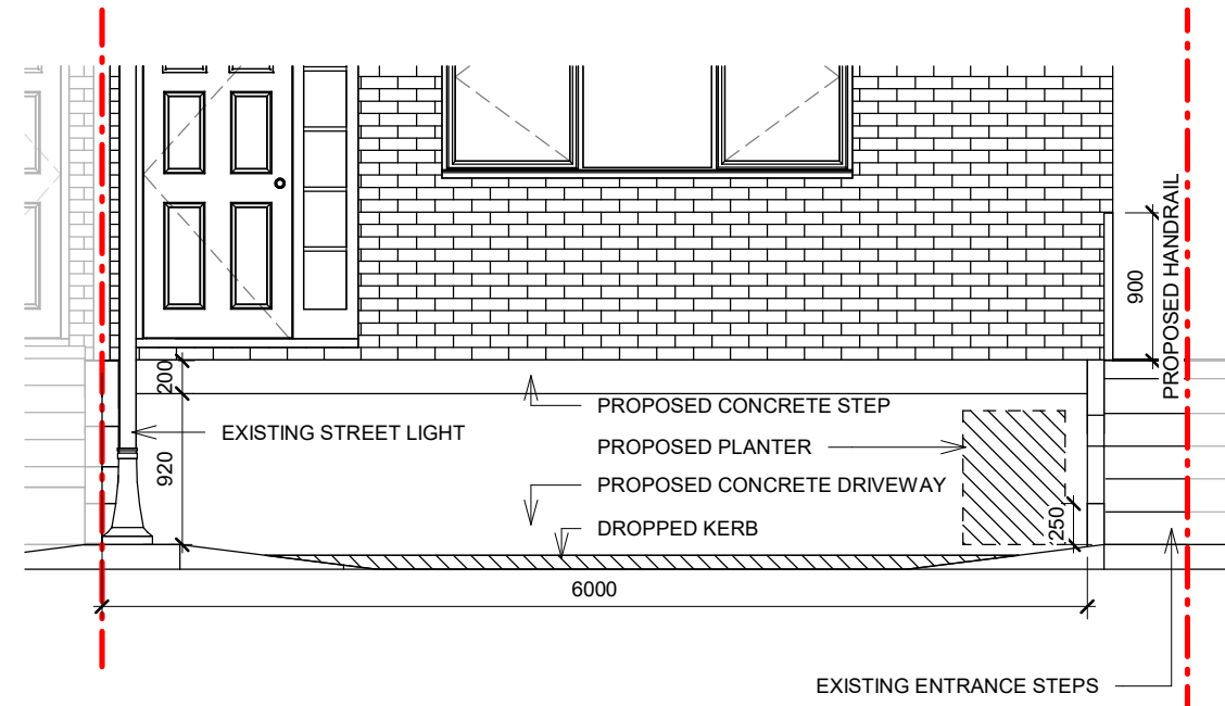
2 FRONT ELEVATION 1:50
