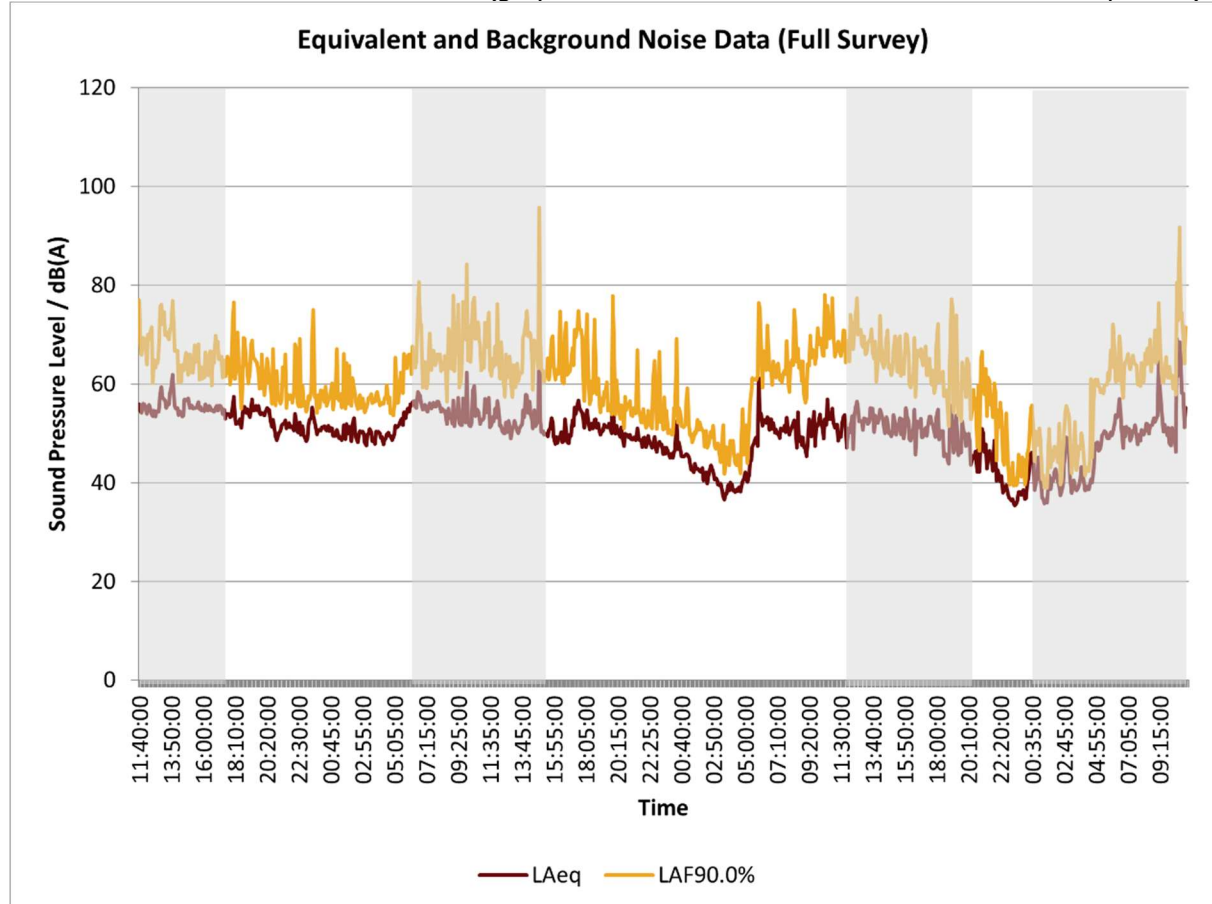
Chart 2: Measured Noise Levels for ML2 (grey sections reflect the adverse weather condition periods)
