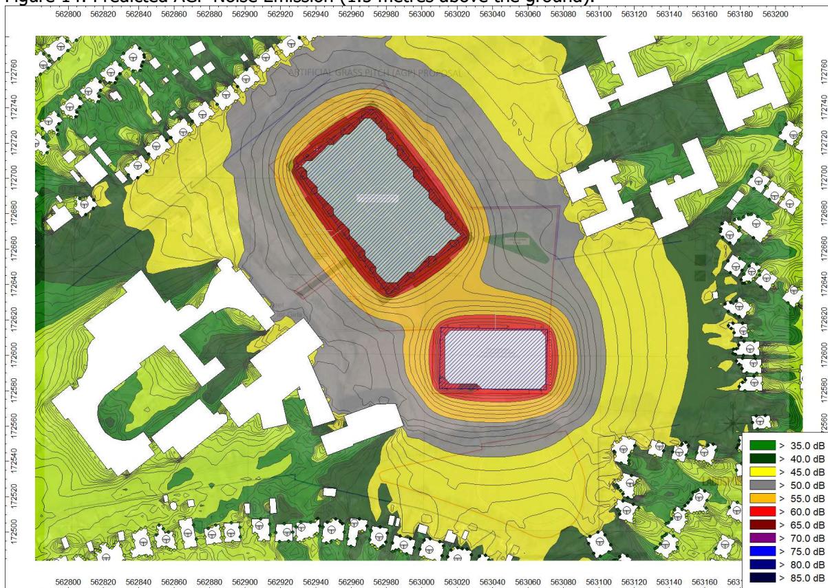
Figure 14: Predicted AGP Noise Emission (1.5 metres above the ground).
