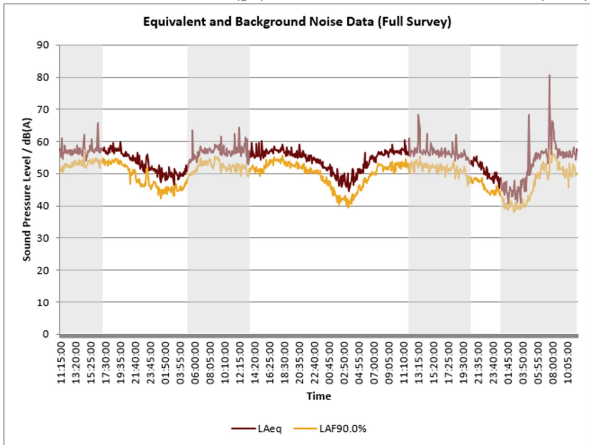
Chart 1: Measured Noise Levels for ML1 (grey sections reflect the adverse weather condition periods)
