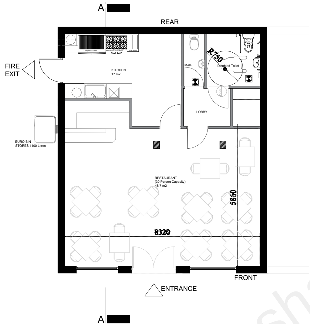
EXISTING GROUND FLOOR PLAN WITH FURNITURE
