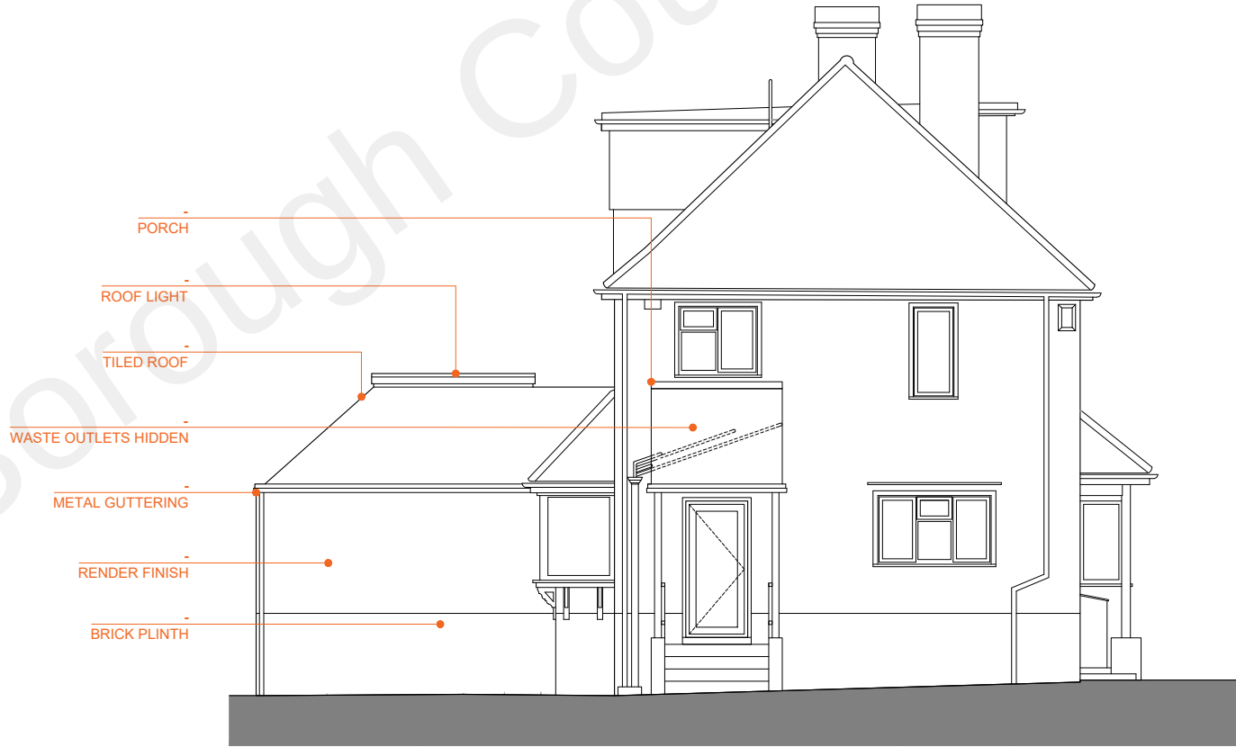
02 PROPOSED NORTH WEST ELEVATION 1:100 @ A3
