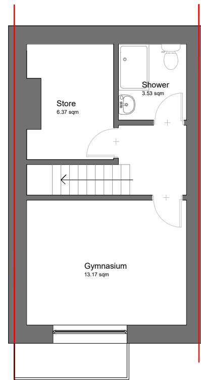
Proposed Basement Floor Plan
