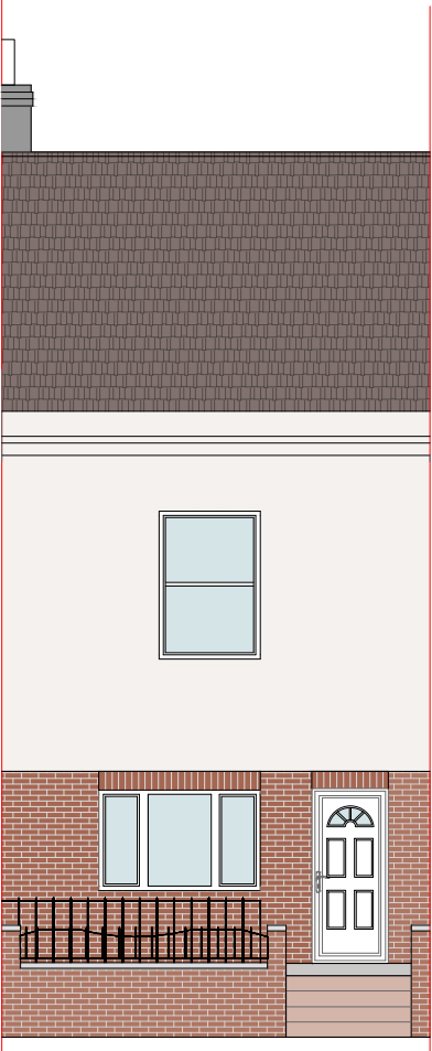
Proposed Front Street Elevation
