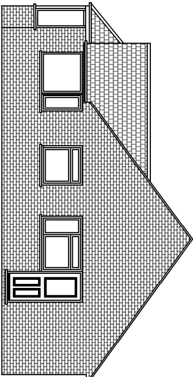
Existing Flank Elevation (B) Scale 1/100
