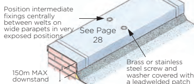
d. Parapet wall capping
