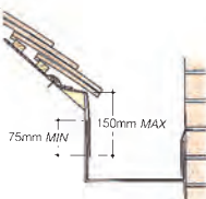
c. Cross section of box gutter
