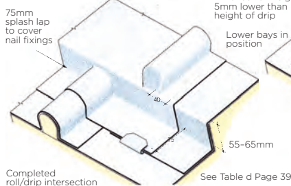
d. Completed roll/drip intersection
