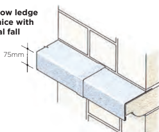
c. Projections with nominal fall
