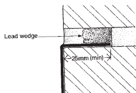
a. Wedging to lead flashing
