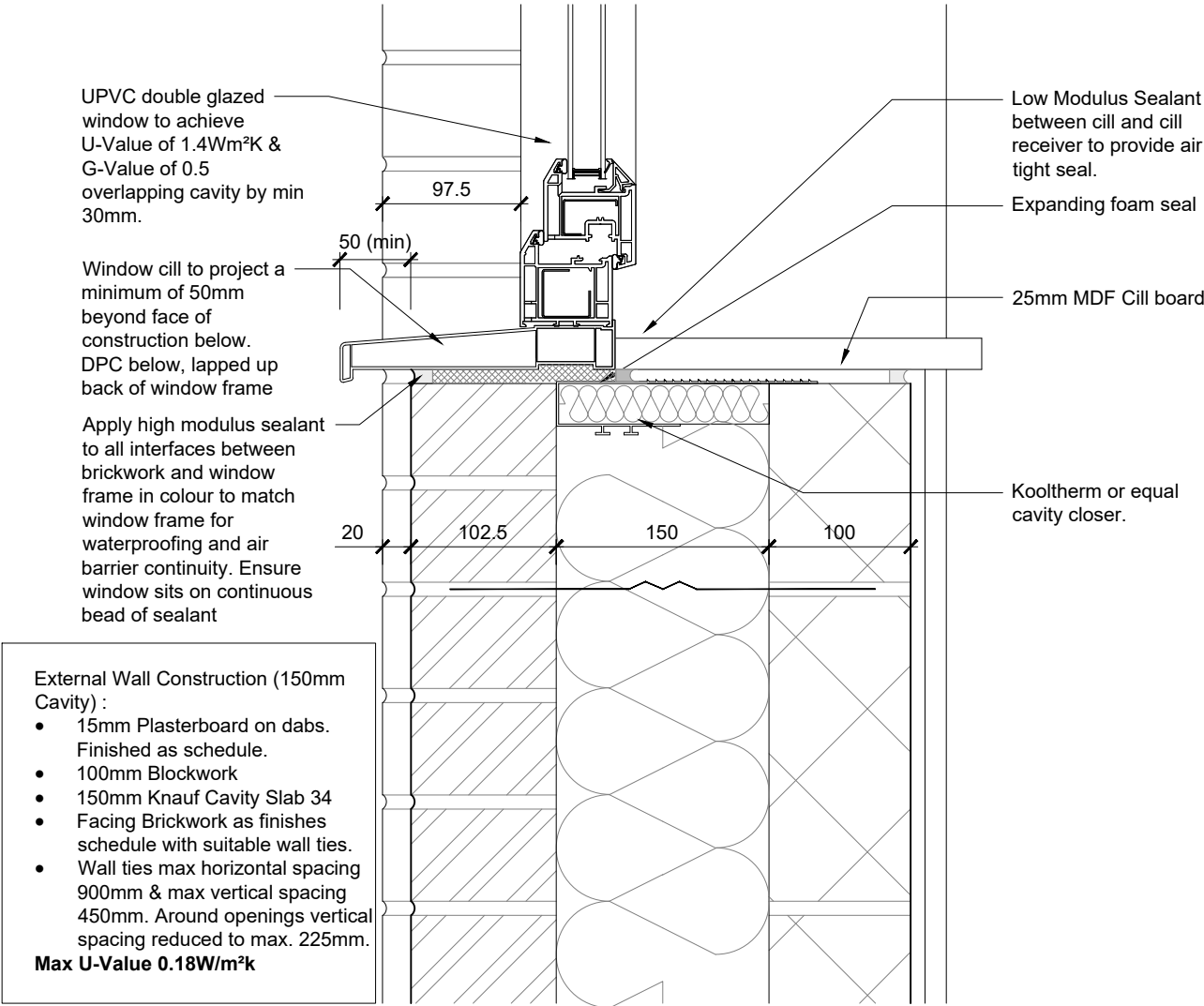
Window Cill - Projected Outer Leaf SCALE 1:5
