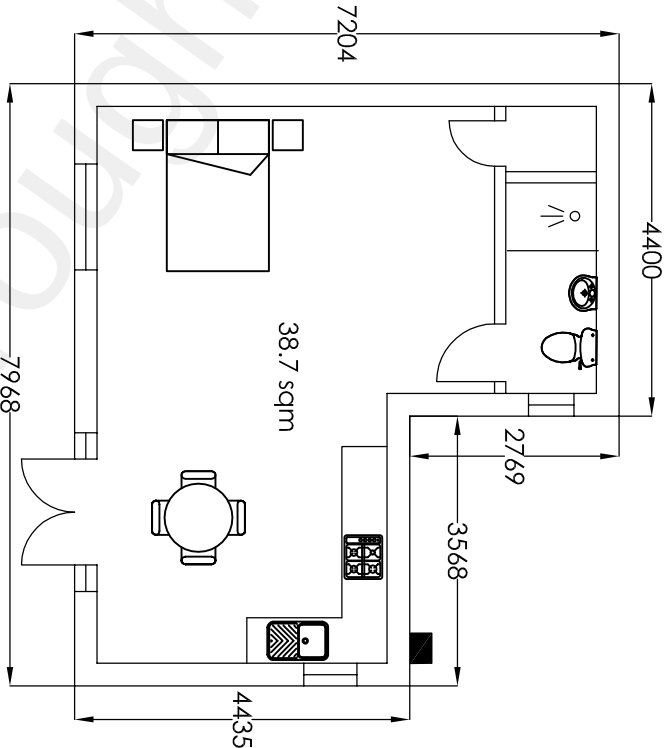
Floor Plan
