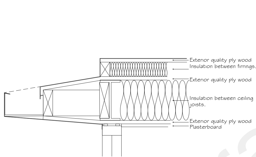
Flat Roof eaves detail Scale 1:10
