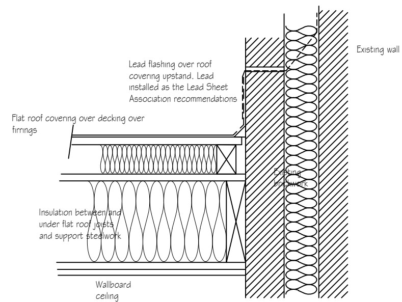
Flat Roof Abutment Scale 1:10
