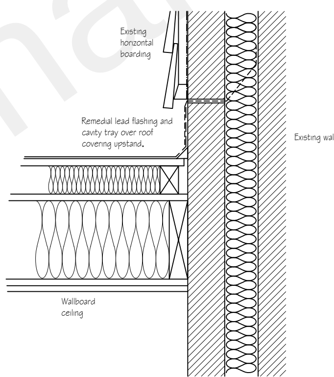
Flat roof abutment Scale 1:10
