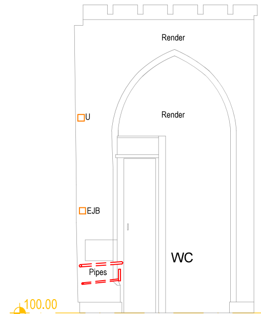
INTERNAL ELEVATION E-5
