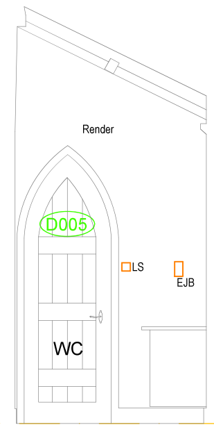
INTERNAL ELEVATION E-6
