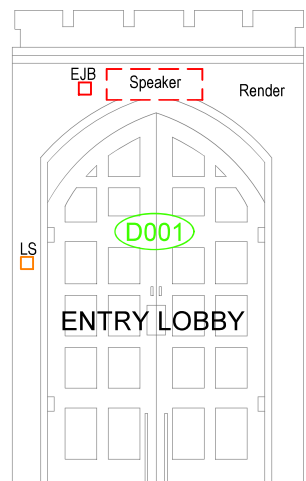
INTERNAL ELEVATION E-11
