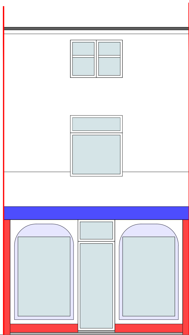
Pre-existing Front Elevation
