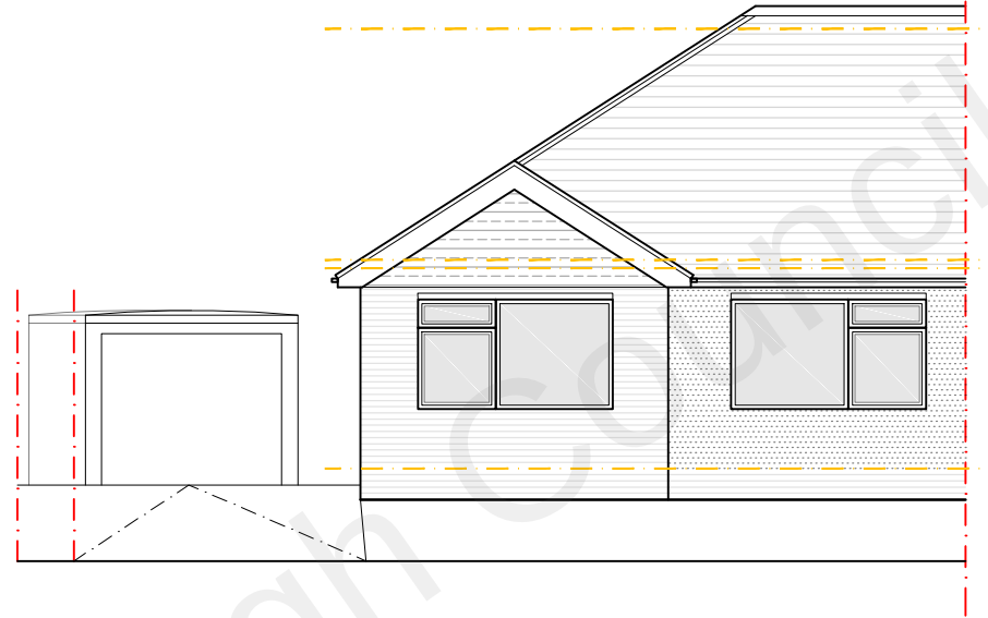
FRONT ELEVATION
