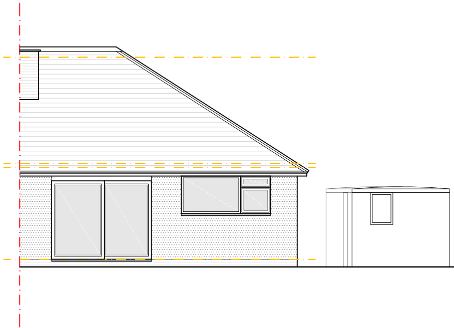
REAR ELEVATION
