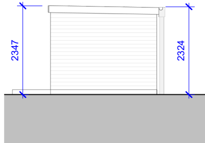
1 160 Summerhouse East Elevation SCALE: 1 : 100
