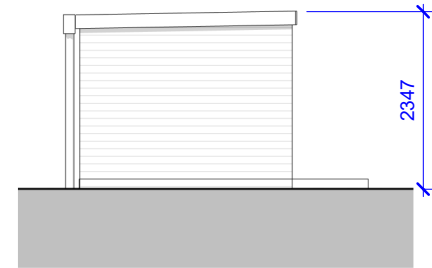
4 160 Summerhouse West Elevation SCALE: 1 : 100
