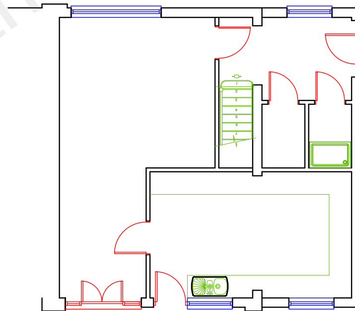
Existing Ground Floor Plan - Scale 1:100@A3
