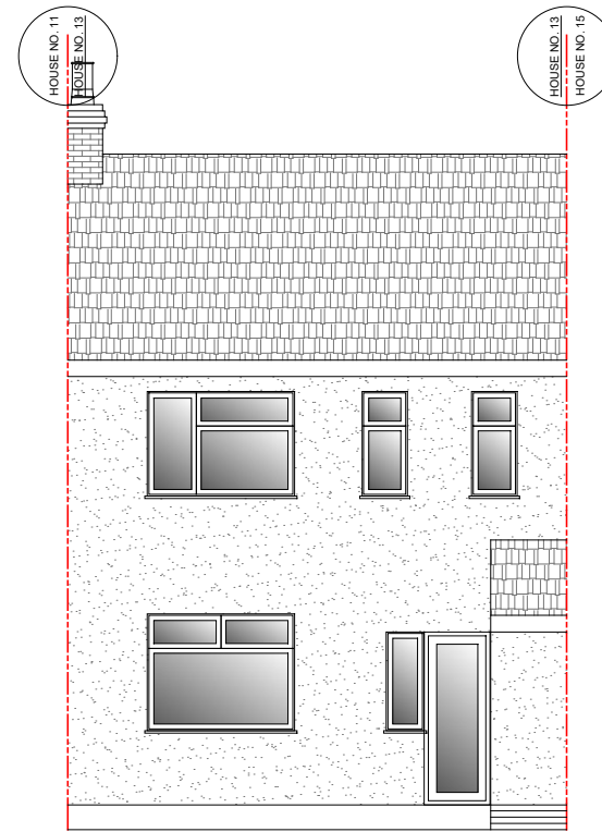
PRE-EXISTING REAR ELEVATION
