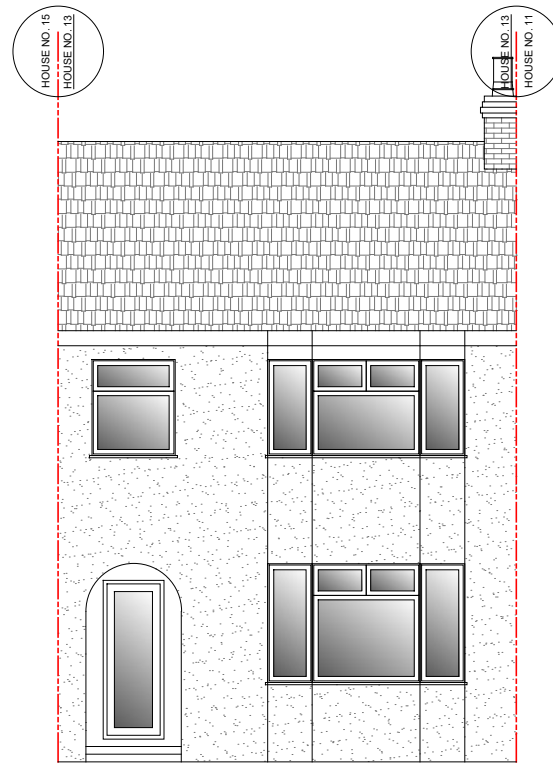
PRE-EXISTING FRONT ELEVATION
