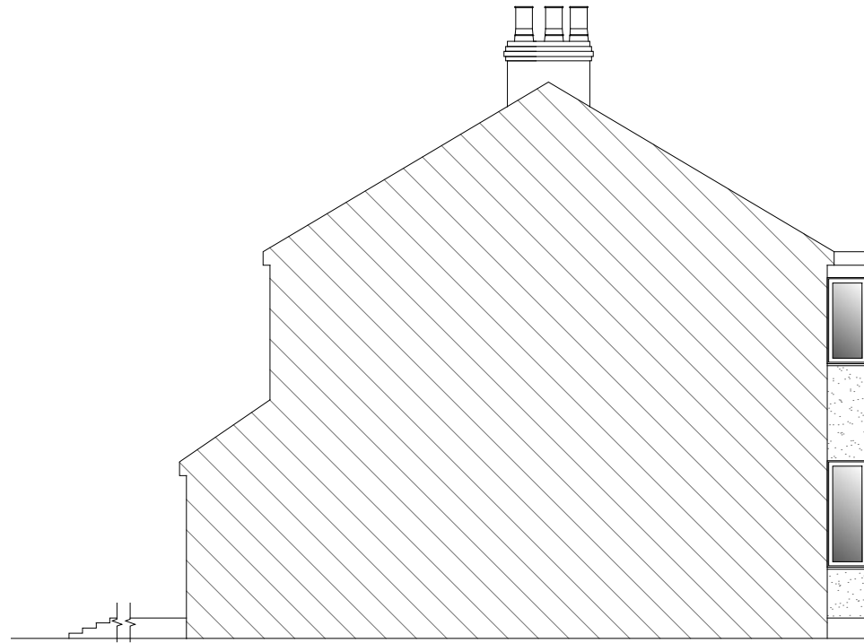
PRE-EXISTING SIDE ELEVATION A
