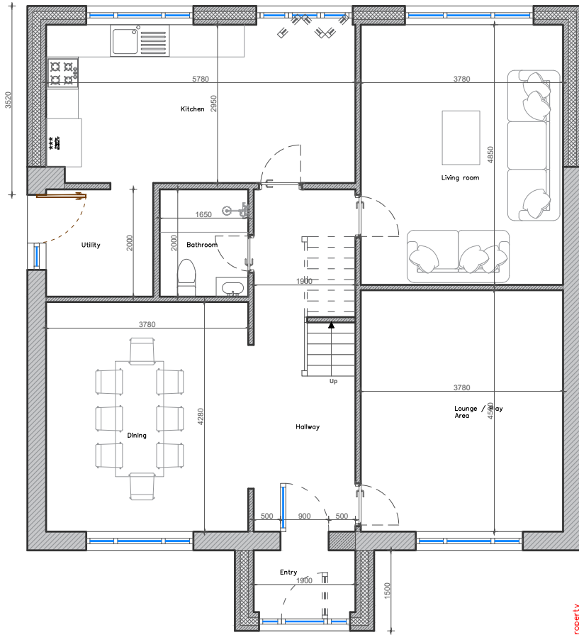
Proposed Ground 1:100
