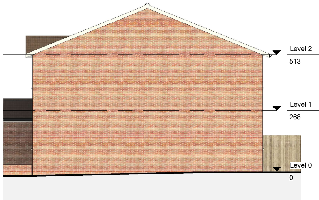
Proposed R Side 1:100
