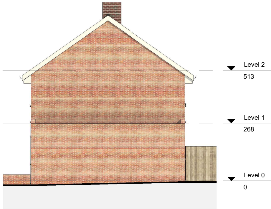
Existing R Side 1:100
