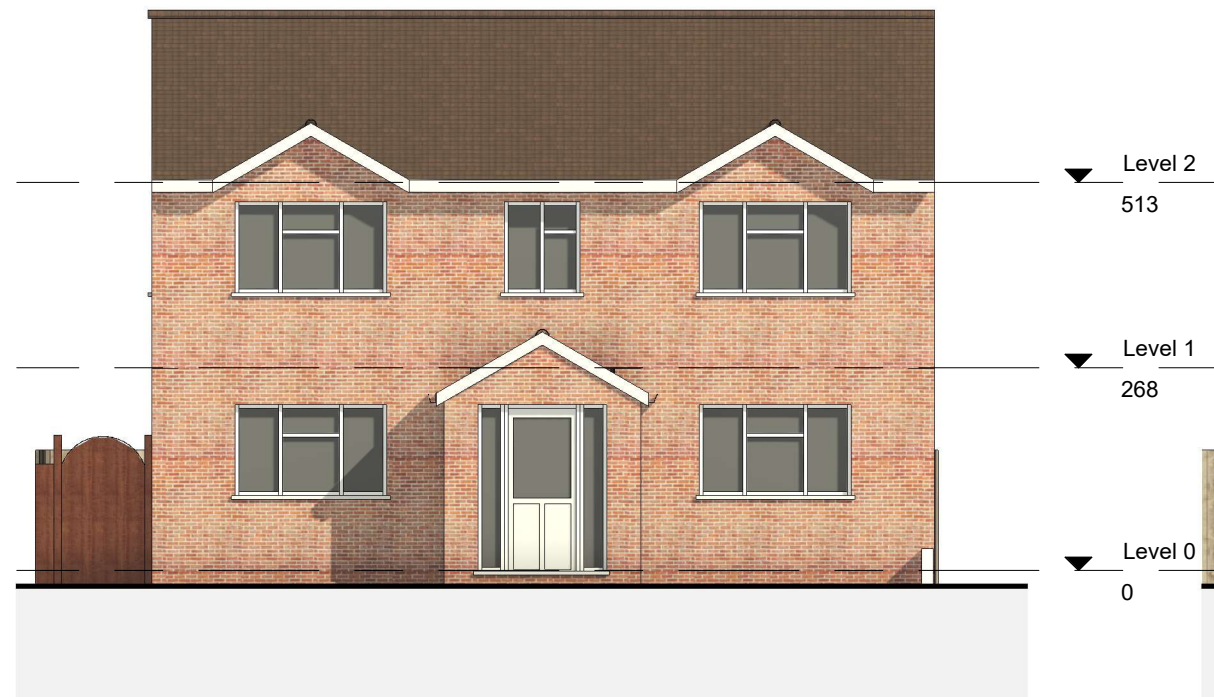
Proposed Front 1:100
